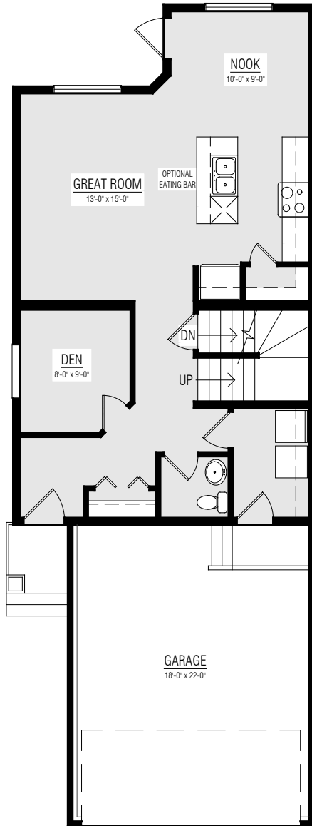
MAIN FLOOR 770 SQ.FT. STANDARD
