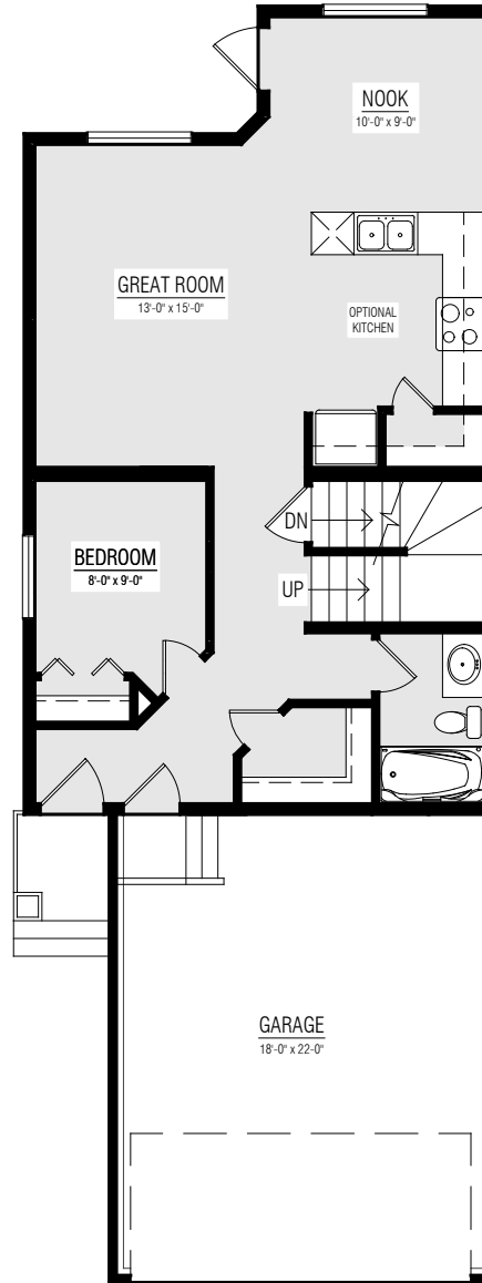
MAIN FLOOR OPTION U-SHAPED KITCHEN & BEDROOM
