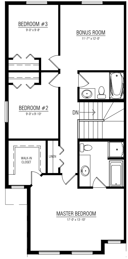
OPTION 2 - REAR BONUS ROOM
